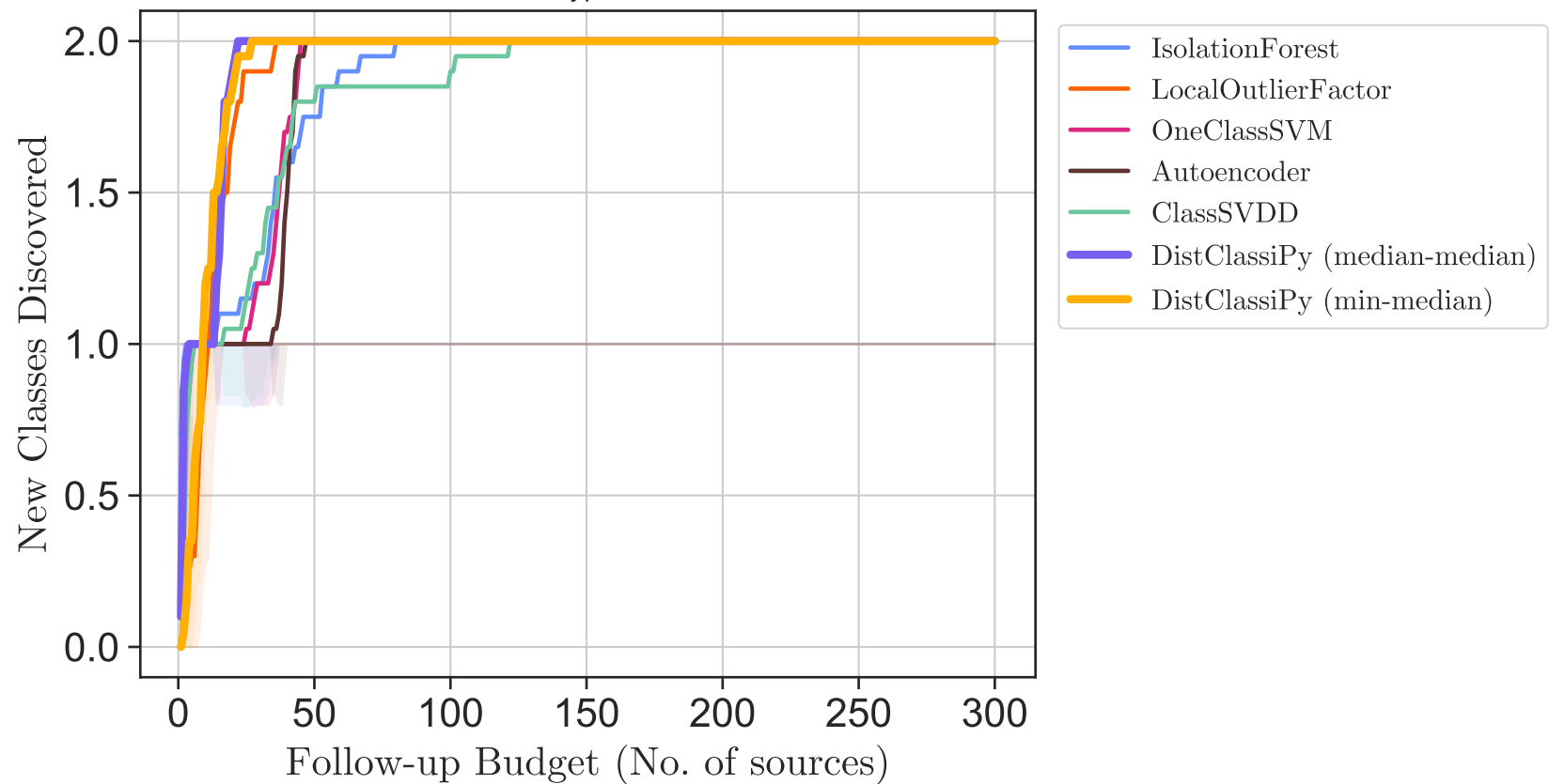
EXP4: Rare Subtype Hunt ELAsTiCC
